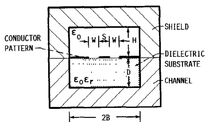
FIGURE 1. - SCHEMATIC ILLUSTRATING A CHANNELIZED COPLANAR WAVEGUIDE (CCPW).
