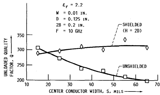
FIGURE 3. - MEASURED UNLOADED QUALITY FACTOR Q FOR CHANNELIZED CPW AS A FUNCTION OF THE CENTER CONDUCTOR WIDTH, WITH AND WITHOUT A SHIELDING ENCLOSURE.
