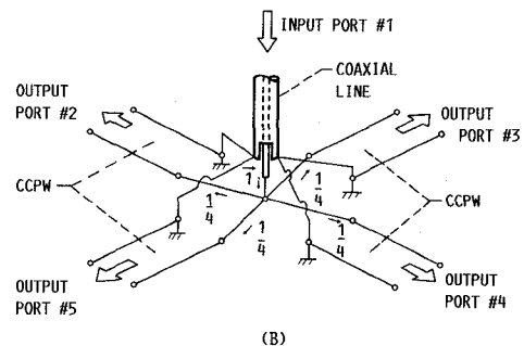
FIGURE 8. - ELECTRIC FIELD ( \vec{E} ) DISTRIBUTION AT THE END OF THE SLOTTED COAXIAL LINE, EQUIVALENT CIRCUIT OF THE JUNCTION SHOWING THE INPUT RF CURRENT ( \vec{I} ) BEING DIVIDED INTO THE FOUR PORTS.
